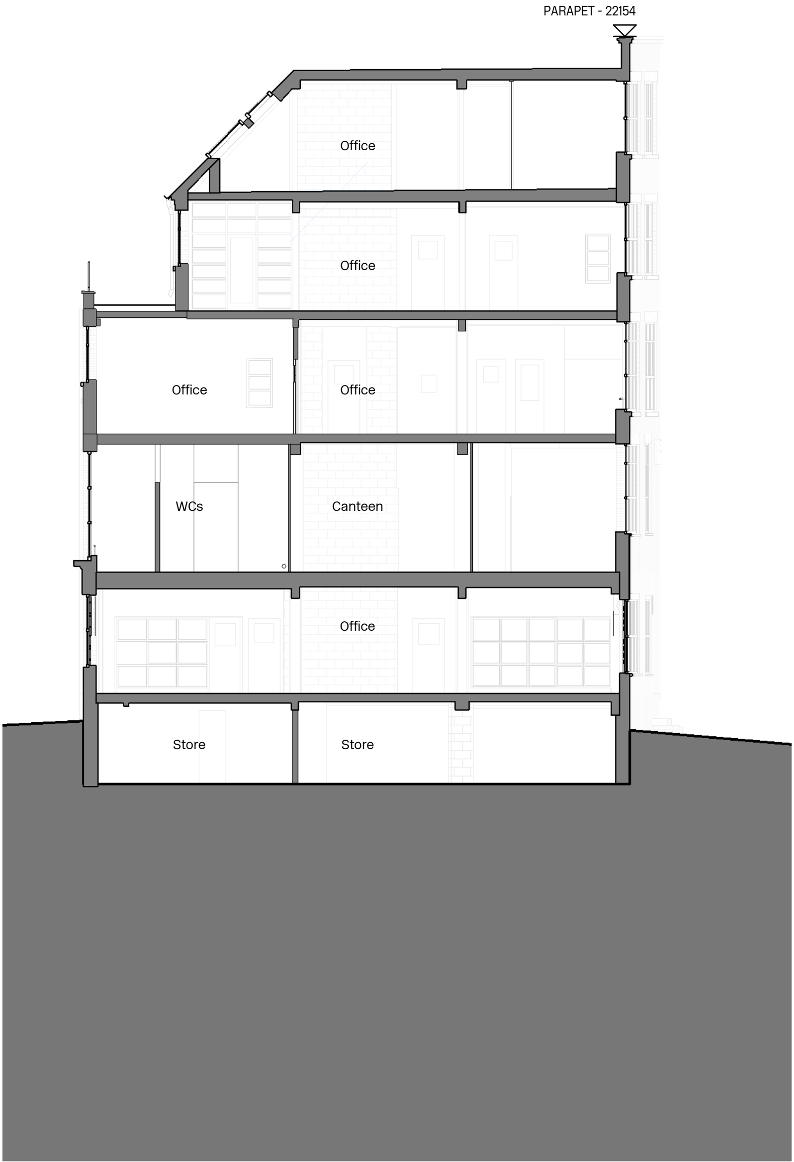
04 Proposed Short Section - Building 04
