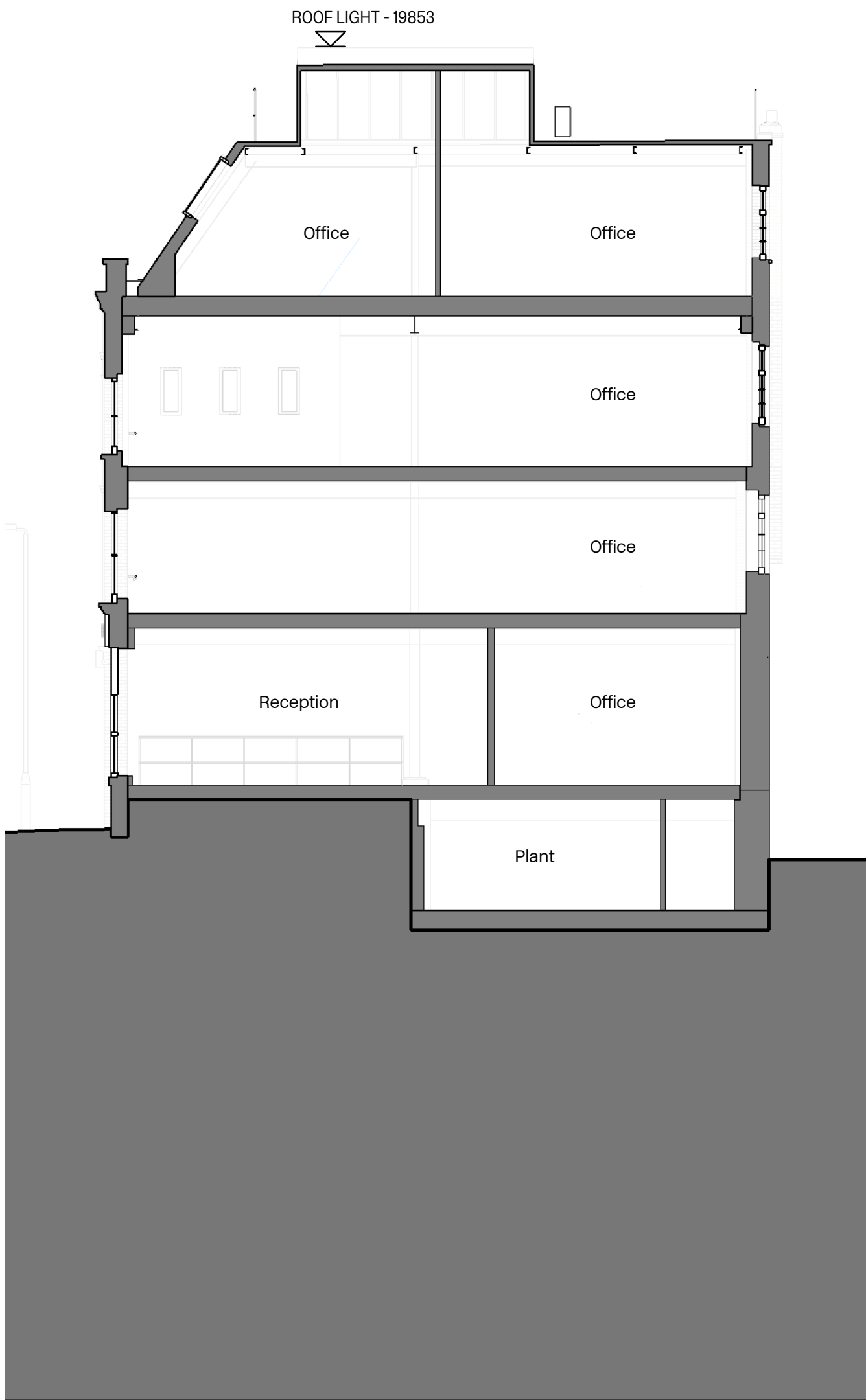
01 Proposed Short Section - Building 01
